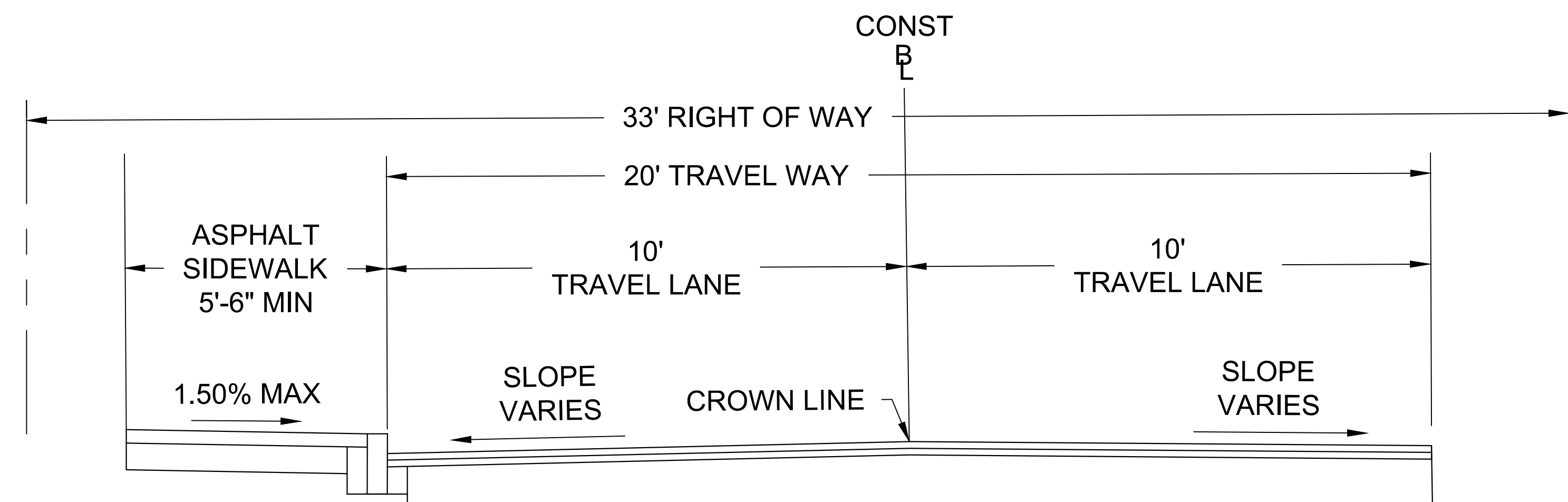
BOWKER STREET SECTION A-A SCALE: NTS
