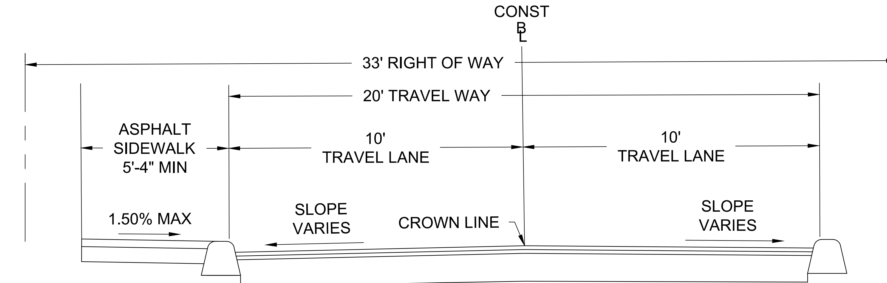
BOWKER STREET SECTION B-B SCALE: NTS
