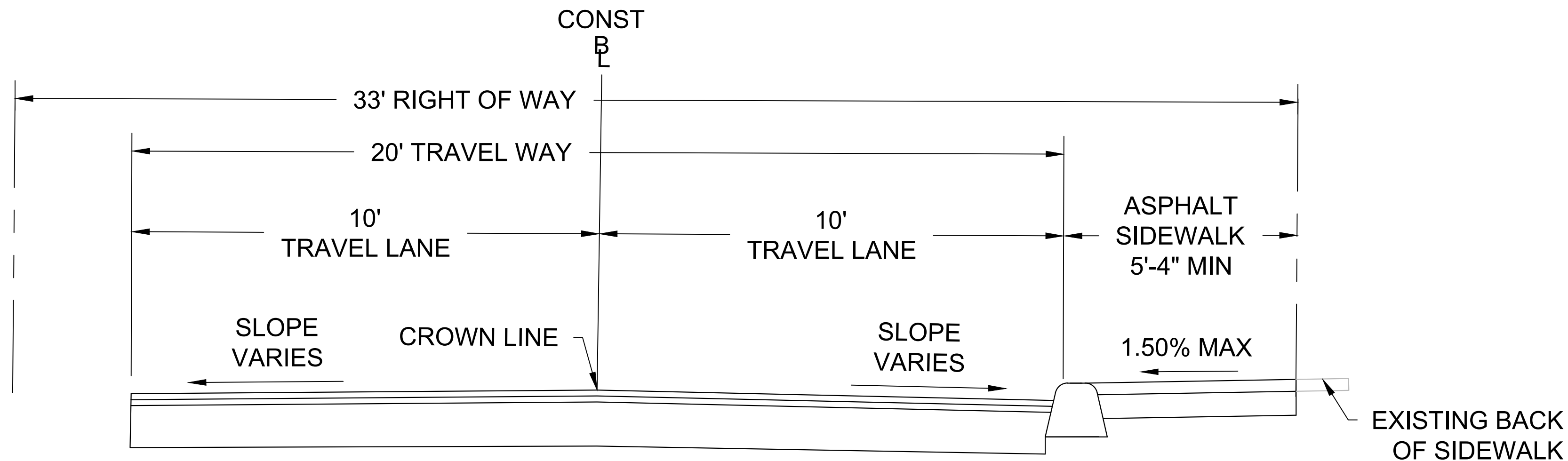
BOWKER STREET SECTION A-A SCALE: NTS
