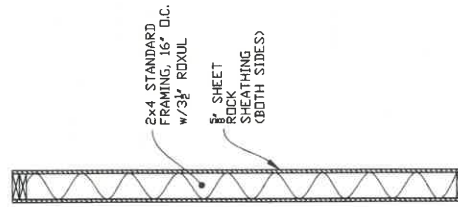
FIRE SEPARATION WALL DETAIL SCALE: 1"=1'
