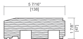
OPTIONAL 1-7/8" SUBSILL
